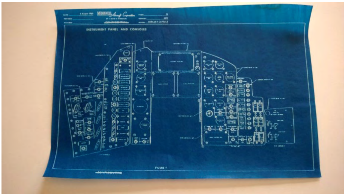
Cyan 36: McDonnell Mercury capsule instrument panel layout
